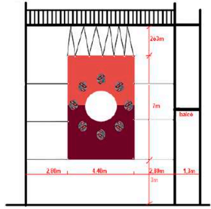
screen scheme
